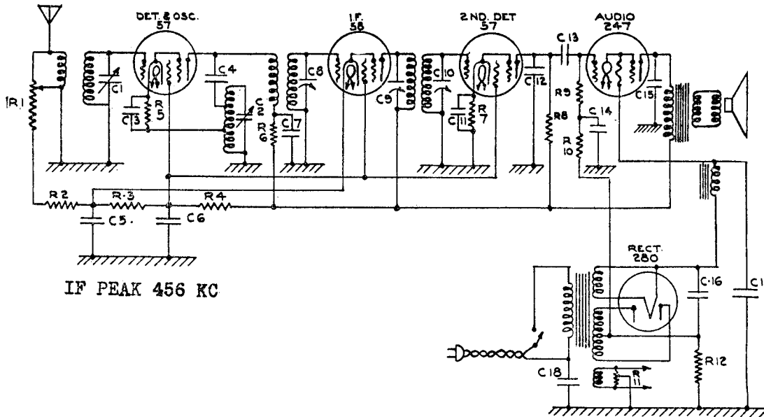
SCHEMATIC WIRING DIAGRAM - MODEL 305A
